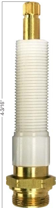
KOHLER® GP30119 Trend/Shore Hot/Cold (OEM) 132389 Hot/Cold ▲102344 Renovation Kit ▲111864 Renovation Kit ▲111865 Renovation Kit ▲111873 O-Ring 128031 Faucet Washer 128451 Bibb Screw ▲128252 Seat ▲120129
