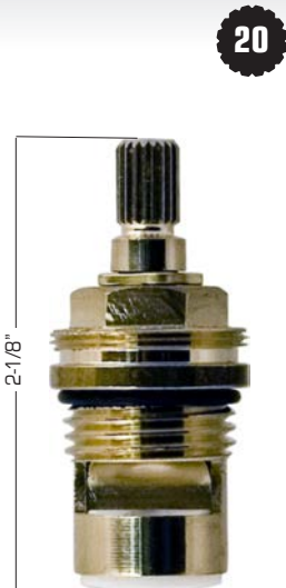
20 ALTMANS / SEARS / UR / PHYLRICH / CONCINNITY Ceramic Disc Hot ▲101632 Cold ▲101682
