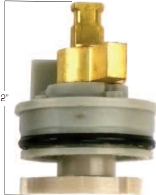
DELTA RP1991 Cartridge 119921, 132351 O-Ring 128044 For Delta® Mix & Scald-Guard®
