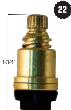
AMERICAN STANDARD 0072950-1700AP • 072951-1700AP Aquaseal
